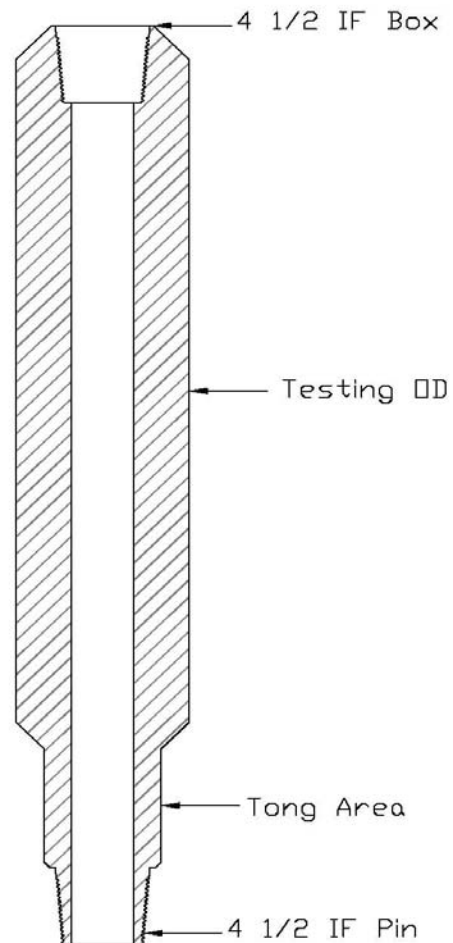
Sub-Sea Casing Ram Test Mandrel (SSCRTM)
