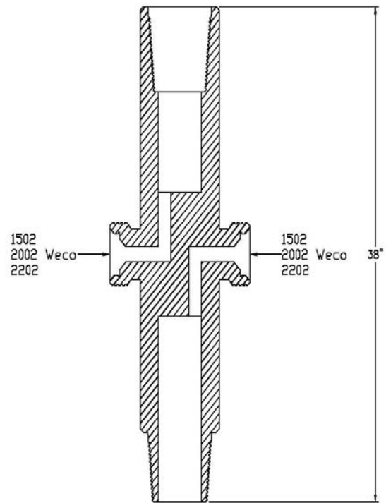
Double Weco Top Test Sub (DWTTs)
