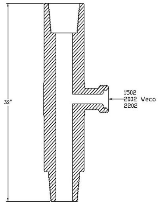
Top Test Sub (TTS)
