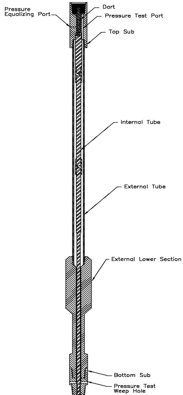
Stack Specific Circulator Test Joint (SSCTJ)
