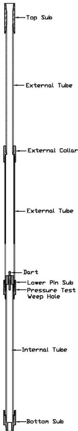
Universal Dynamically Positioned Stack Specific Test Joint (Tool Stroked Open)
