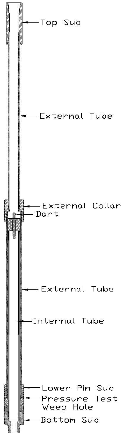
Universal Dynamically Positioned Stack Specific Test Joint (Tool Stroked Closed)
