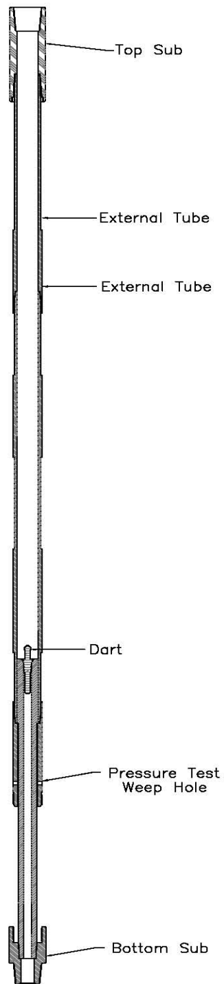
Dynamically Positioned Stack Specific Test Joint (Tool Stroked Open)
