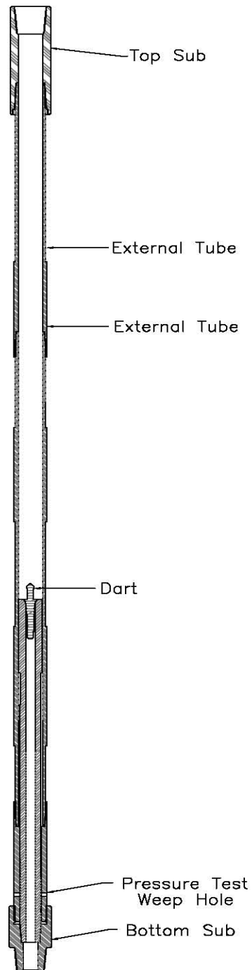
Dynamically Positioned Stack Specific Test Joint (Tool Stroked Closed)
